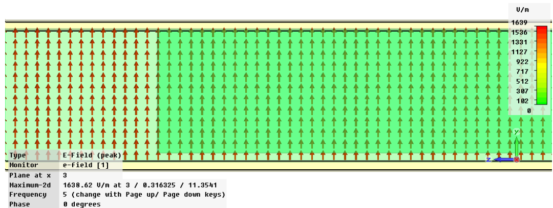
Figure 179 E-field plot at cross section X = 3.0 mm and frequency 5 GHz
