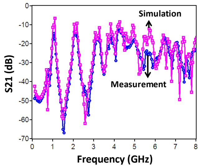
Figure 63 Comparison of simulation and measurement results for the structure in Figure 62 without EBGs on M3
