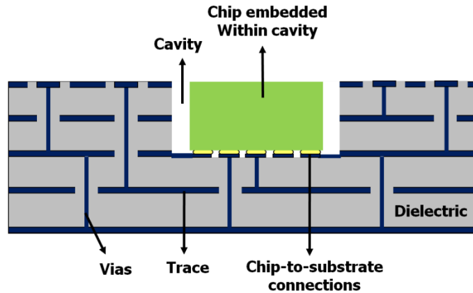
Figure 9 Chip-last embedded chip package
