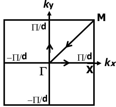
Figure 75 Brillouin zone for a unit cell of square shape and size d
