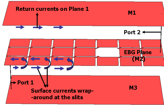
Figure 51 EBG plane sandwiched between two isolated planes
