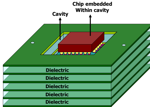
Figure 5 Package with embedded chip
